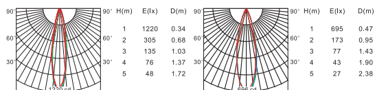
Beam angle 30° Output power 3W Luminous flux 216lm
