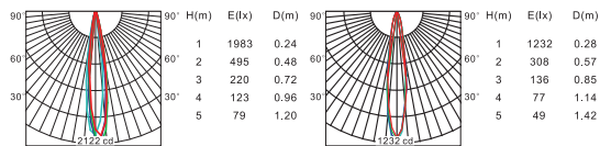
Beam angle 15° Output power 3W Luminous flux 210lm
